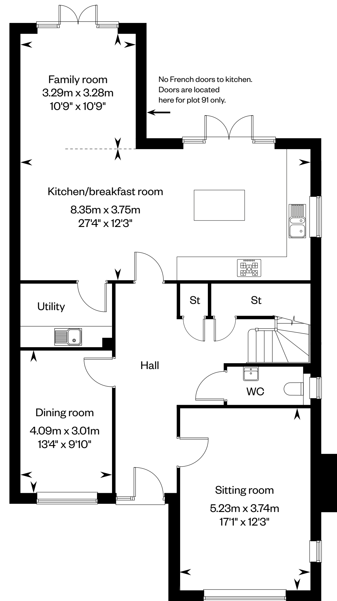
Ground floor
