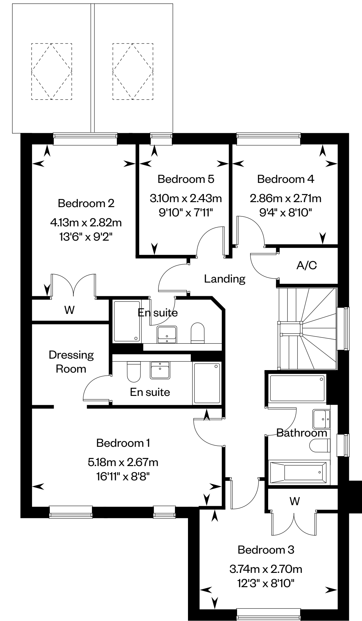
First floor
